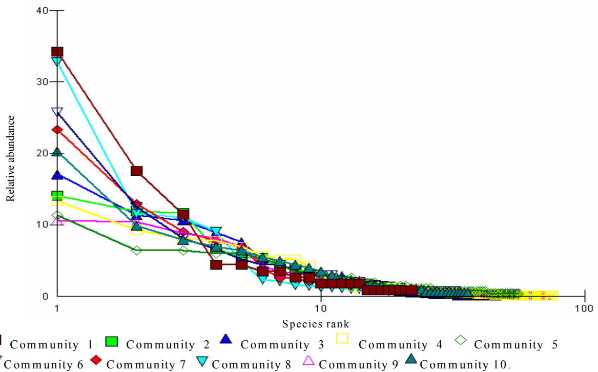
Figure 5.4 Rank-abundance curves showing trees species dominance across communities in Mpigi forests
